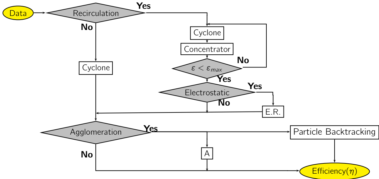
Figure 6: Representation of the different models integration
