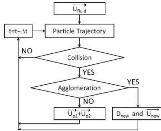
Figure 4: Representation of interparticle agglomeration model
