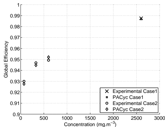
Figure 9: Global efficiency at several concentrations for pilot scale: experimental and PACyc predictions
