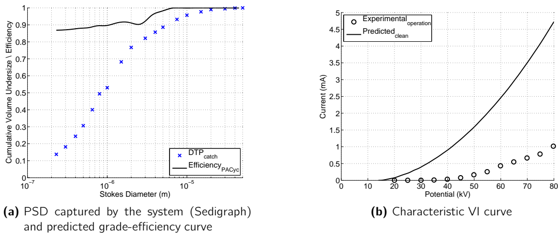
Figure 11: Case 4 - ReCyclone ® EH industrial application example: straw fired boiler
