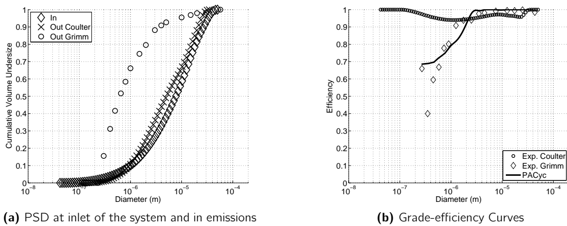
Figure 8: Case 2 - waste of a vertical lime furnace for cement production
