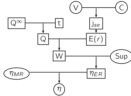
Figure 3: Information flow diagram to illustrate the internal operations of the electrical model
