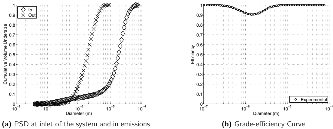
Figure 10: Case 3 - ReCyclone ® MH industrial application example: biomass heated corkwood boiler
