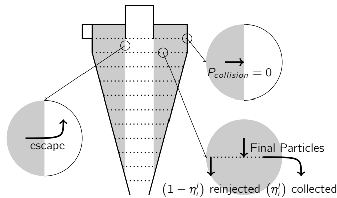
Figure 5: Properties of particles in different zones of the reverse-flow gas cyclone
