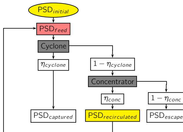
Figure 2: Iterative process concerning the processed particle size distribution
